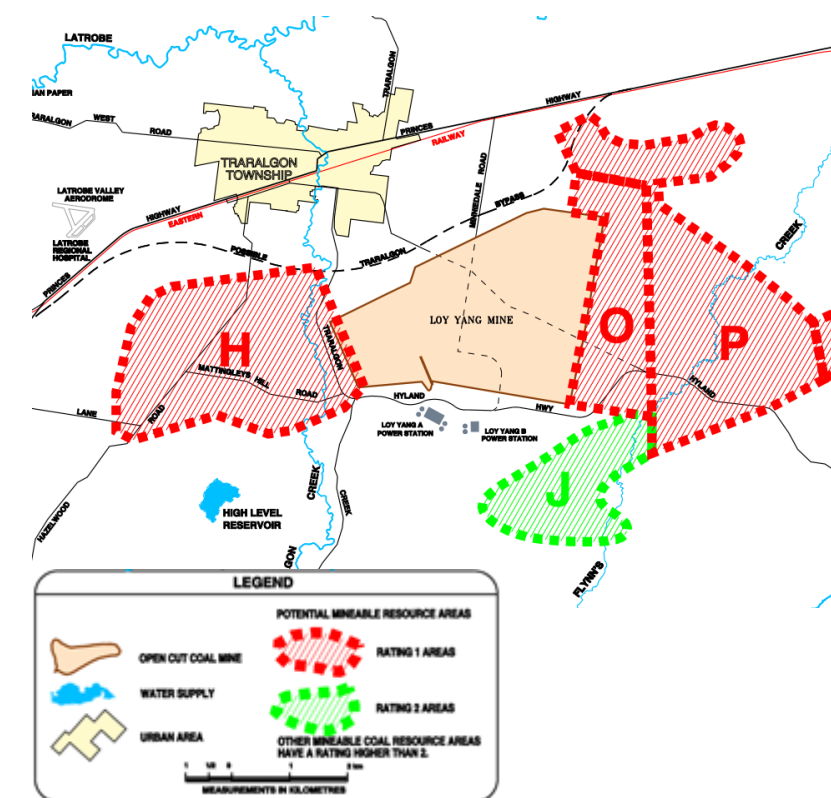
Figure 19: map of highly rated coal areas
