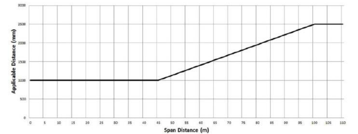
GRAPH 2: UNINSULATED LOW VOLTAGE ELECTRIC LINE IN LOW BUSHFIRE RISK AREA
