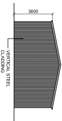
SOUTH ELEVATION
