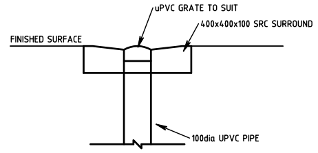
DETAIL - INSPECTION OPENING
