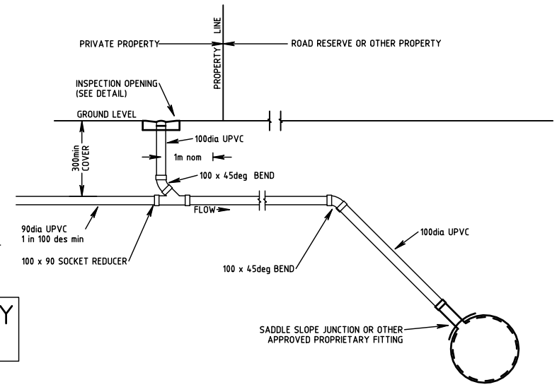
SECTION ALONG PROPERTY CONNECTION
