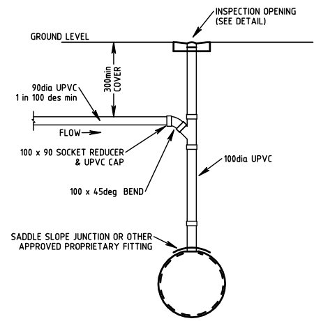
SECTION ALONG PROPERTY CONNECTION
