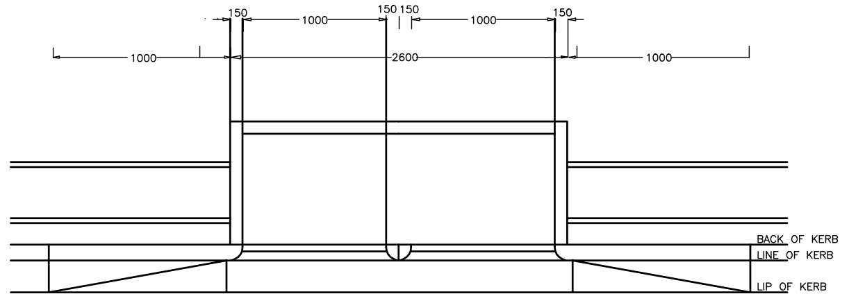
PLAN (COVER REMOVED)
